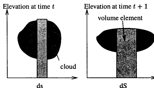
Figure 4: Conservation of cloud between two dates.
